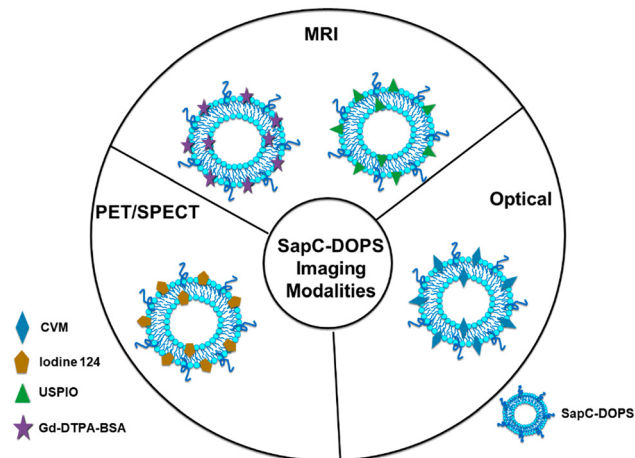
Fig. 6 Schematic diagram showing that many imaging modalities use saposin C-dioleoyl phosphatidylserine (SapC-DOPS)-based modalities to visualize tumors. The far-red fluorophore CVM can be attached to the SapC-DOPS nanovesicles to provide optical imaging for both in vivo and in vitro studies. The use of gadolinium chelates, such as ultrasmall superparamagnetic iron oxide (USPIO) or gadolinium-DTPA-bis (stearyl amide) (Gd-DTPA-BSA), as MRI contrast agents is necessary to enable in vivo MRI. Moreover, SapC-DOPS combined with an iodine-124 contrast agent is used for in vivo PET/SPECT imaging. Reprinted from, ref. 18 Copyright CC BY 2022 MDPI.
