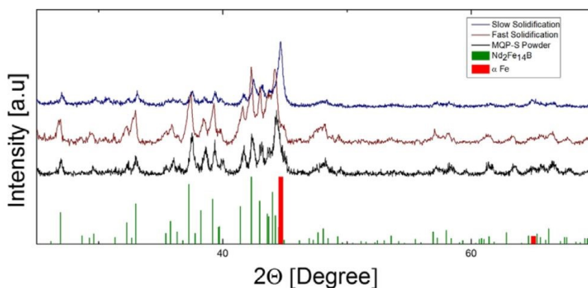
Figure 16 XRD patterns of LPBF-processed NdFeB samples – Initial feedstock powder, samples processed at different rates of solidification, theoretical spectra of Nd 2 Fe 14 B and \alpha Iron (added as guidance) [6]
