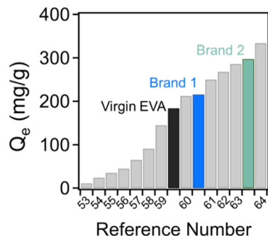
Fig. 10 Comparison of the equilibrium adsorption capacity of the shoe-waste-derived materials to the results found in ref. 53–64.
