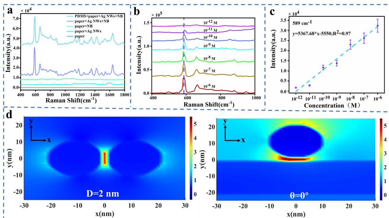
Fig. 2 SERS spectra (a) on various papers and (b) of NB with different concentrations; (c) the linear fitting curve of Raman intensities at 589 \text{ cm}^{-1} ; (d) simulated electric field distribution of the AgNW dimer.
