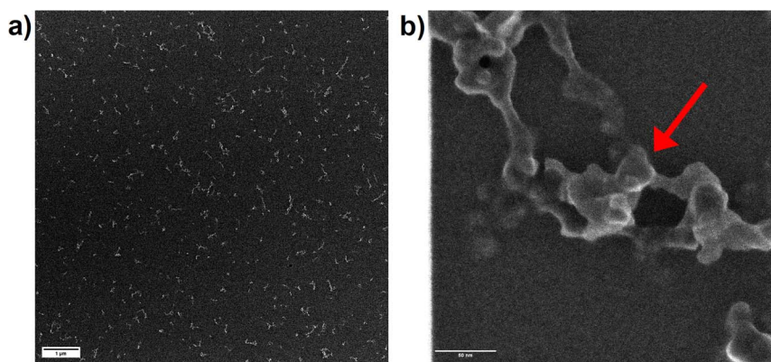
Fig. 10 (a) Secondary electron images of the laser-generated aerosol formed in argon visualized by scanning transmission electron microscopy with the scale bar size set at 1\ \mu\text{m} . (b) Higher magnification of a single agglomerate enabling with the scale bar set at 50\ \text{nm} and a red arrow was added to indicate a preliminary particle.
