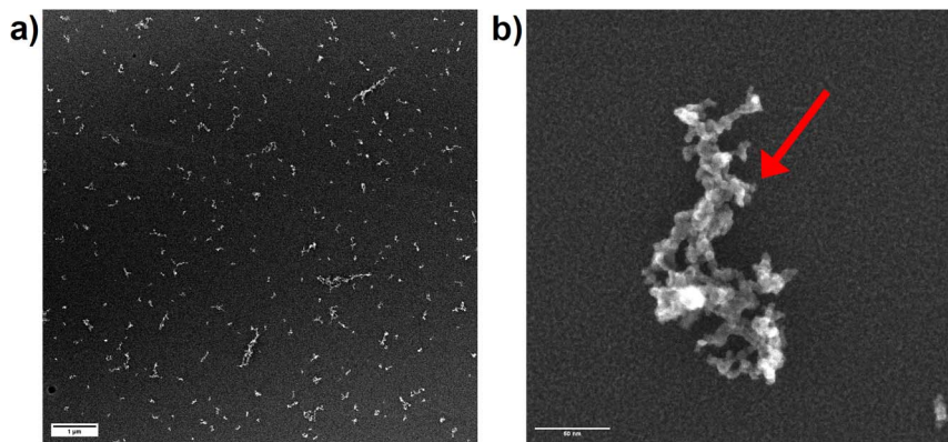
Fig. 9 (a) Secondary electron images of the laser-generated aerosol formed in nitrogen visualized by scanning transmission electron microscopy with the scale bar size set at 1\ \mu\text{m} . (b) Higher magnification of a single agglomerate enabling the identification of the primary particles with the scale bar set at 50\ \text{nm} and a red arrow was added to indicate a preliminary particle.
