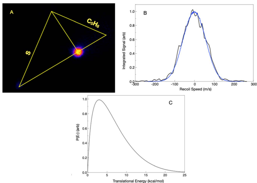
Fig. 6 (A) Velocity map image of the 99 u product, \text{C}_5\text{H}_7\text{S} , for the reaction of \text{S}(^3\text{P}) with isoprene (Newton diagram superimposed) under a collision energy of 14.0 kcal mol ^{-1} . (B) Total signal from the image in (A) projected onto the x -axis and transformed into a speed distribution (black). The simulated image using the velocity distribution is then projected to produce a profile (blue) that closely matches the observed one. (C) Total translational energy release ( P(E_T) ) extracted following analysis of the image in (A).
