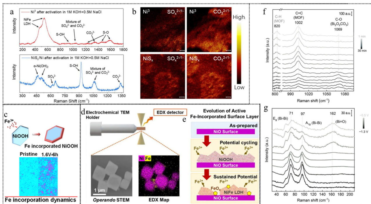
Fig. 15 (a) Raman spectra of \text{Ni}^3 and \text{NiS}_x/\text{Ni} after 12-h activation in 1 \text{ M KOH} + 0.5 \text{ M NaCl} . (b) TOF-SIMS map of \text{SO}_x^{2-/1-} and \text{CO}_3^{2-/1-} fragments from a \text{Ni}^3 and \text{NiS}_x/\text{Ni} electrode surface after activation in 1 \text{ M KOH} + 0.5 \text{ M NaCl} at 400 \text{ mA cm}^{-2} . This figure has been reproduced from ref. 33 with permission from National Academy of Science, copyright 2023. (c) Pristine \text{Ni(OH)}_2 , \text{Ni(OH)}_2 after 6 h CA measurement at 1.6 \text{ V} vs. RHE in 1 \text{ M KOH} containing 10 \mu\text{M Fe}^{3+} . This figure has been reproduced from ref. 137 with permission from American Chemical Society, copyright 2021. (d) In situ STEM schematic setup and images and STEM/Fe EDX maps of NiO octahedra acquired in a 0.5 \text{ M} borate buffer +1 \text{ mM Fe(NO}_3)_3 solution. (e) Illustration of the evolution of Fe incorporated surface reconstruction. This figure has been reproduced from ref. 138 with permission from American Chemical Society, copyright 2023. In situ Raman spectra revealing the conversion from (f) Bi-MOF NR to \text{Bi}_2\text{O}_2\text{CO}_3 NS on exposure to 0.1 \text{ M KHCO}_3 and (g) \text{Bi}_2\text{O}_2\text{CO}_3 NS to Bi NS under CRR conditions. This figure has been reproduced from ref. 139 with permission from Wiley-VCH, copyright 2021.
