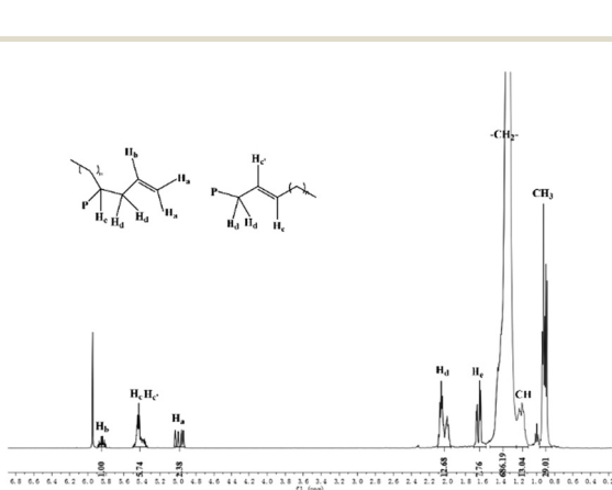
Fig. 9 ^1\text{H} NMR spectrum of the polyethylene sample produced using Ni5/EASC at 20 °C (entry 5, Table 4), recorded at 110 °C in 1,1,2,2-tetrachloroethane- d_2 .
