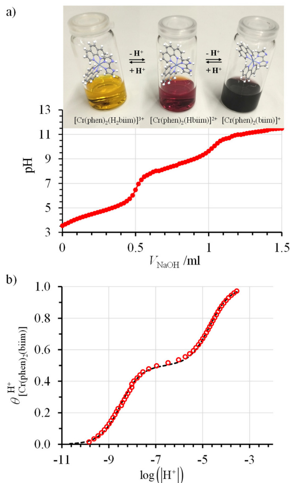
Fig. 8 (a) Titration of 51 mg (52 \mu\text{mol} ) of [\text{Cr}(\text{phen})_2(\text{H}_2\text{biim})](\text{CF}_3\text{SO}_3)_3 (10 mL aqueous \text{KNO}_3 0.1 M, c = 5.2 \text{ mmol L}^{-1} ) with \text{NaOH} 0.1 N highlighting the color changes and (b) associated binding isotherm depicted as plots of experimental (red circles, eqn (5)) and fitted (dashed black trace, eqn (8)) occupancy factors as a function of \log([\text{H}^+]) .
