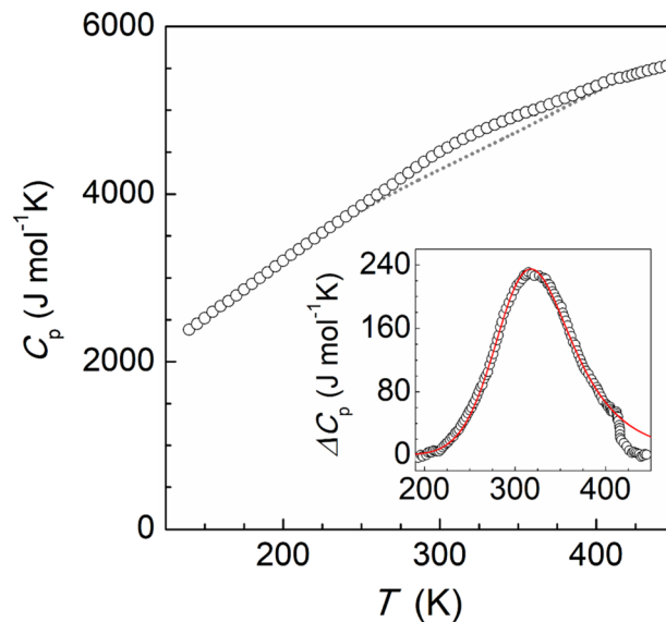
Fig. 5 Molar heat capacities of compound 2. The dashed line represents the estimated normal heat capacities used for \Delta C_p determination. Inset: excess heat capacity and its simulation using Sorai domain model (see text).
