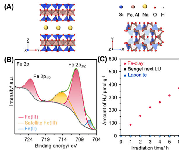
Fig. 20 (A) Polyhedral model of the smectite structure from the [100] direction and [001] direction, (B) Fe 2p XPS spectrum of Fe-clay, and (C) photocatalytic H 2 evolution of Fe-clay (red circle), Bengel next LU (black square), and LAPONITE® (blue triangle) from aqueous MeOH. 386
