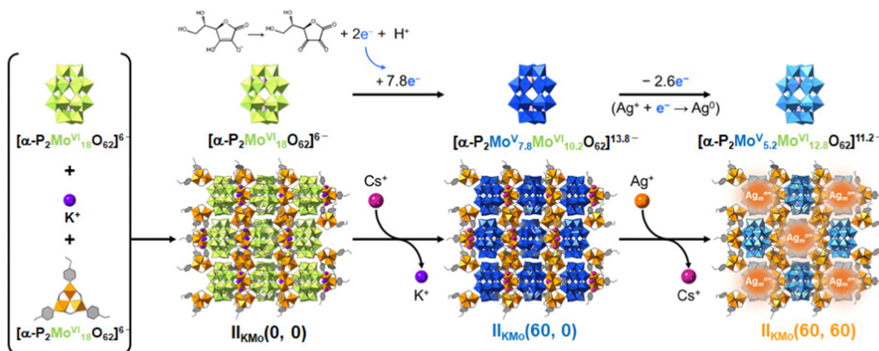
Fig. 8 Schematic representation of the Ag cluster formation in a PIC scaffold. Relationship among as-synthesized PIC ( \text{II}_{\text{KM}0}(0, 0) ), reduction-induced ion-exchange of \text{K}^+ with \text{Cs}^+ ( \text{II}_{\text{KM}0}(60, 0) ), and Ag incorporation followed by Ag cluster formation ( \text{II}_{\text{KM}0}(60, 60) ). \text{II}_{\text{KM}0}(t_1, t_2) represents the PIC, which has been reduced and ion-exchanged with \text{Cs}^+ for t_1 min followed by the immersion in aqueous solution of \text{AgNO}_3 for t_2 min. Note that the number of transferred electrons with decimal points ( 7.8\text{e}^- and 2.6\text{e}^- ) indicates bulk averages. Reprinted with permission from Haraguchi et al. Copyright 2023 Wiley-VCH.
