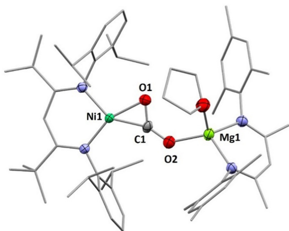
Fig. 3 Molecular structure of 3 . H atoms and co-crystallised solvent molecules omitted for clarity. Selected bond lengths (Å) and angles ( ^\circ ): Ni1–C1 1.839(2), Ni1–O1 1.925(2), C1–O1 1.269(4), C1–O2 1.236(3), O1–C1–O2 129.3(3), O2–Mg1 1.974(2).
