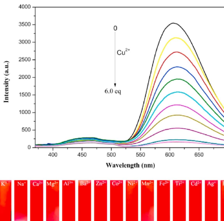
Fig. 14 Emission spectra of probe 9 upon increasing concentrations of \text{Cu}^{2+} ions in \text{THF}/\text{H}_2\text{O} mixtures ( v/v = 1:9 , \text{pH} = 7.4 , \lambda_{\text{ex}} = 350 \text{ nm} ) (top) and photographs of the silica gel testing strips for detecting various ions including under UV 365 nm illumination (bottom). Reproduced with permission from ref. 54. Copyright 2022 Elsevier.
