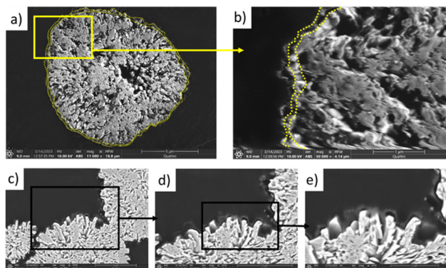
Fig. 5 SEM of a cross-sectioned NMC-B particle (a), the dotted lines represent the LiAlO 2 coating layer. The framed region shows a zoom on the LiAlO 2 coating layer (b). Cross-section of another NMC-B particle (c). The framed region shows a zoom on the LiAlO 2 coating layer (d and e).
