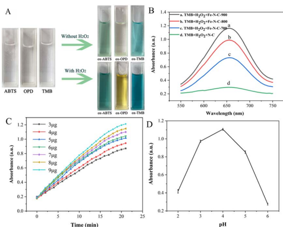
Fig. 4 (A) Dual response enzyme-mimicking activity; (B) effect of materials on the catalytic efficiency of Fe-N-C; (C) time-dependent absorbance changes of the reaction system for different Fe-N-C concentrations; (D) effect of pH on the catalytic efficiency of Fe-N-C.
