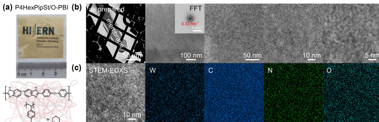
Fig. 3 (a) Image of the blend membrane with a P4HexPipSt content of 73 wt% and structure of the blend components. (b) HAADF-STEM images of the as prepared membrane. (c) STEM-EDX spectrum images showcasing the initial homogeneous distribution of C, N, and O, as well as W utilized for staining. Structure size within the membrane was evaluated via the radial profile of the fast Fourier transformed micrograph (FFT) shown in (b).
