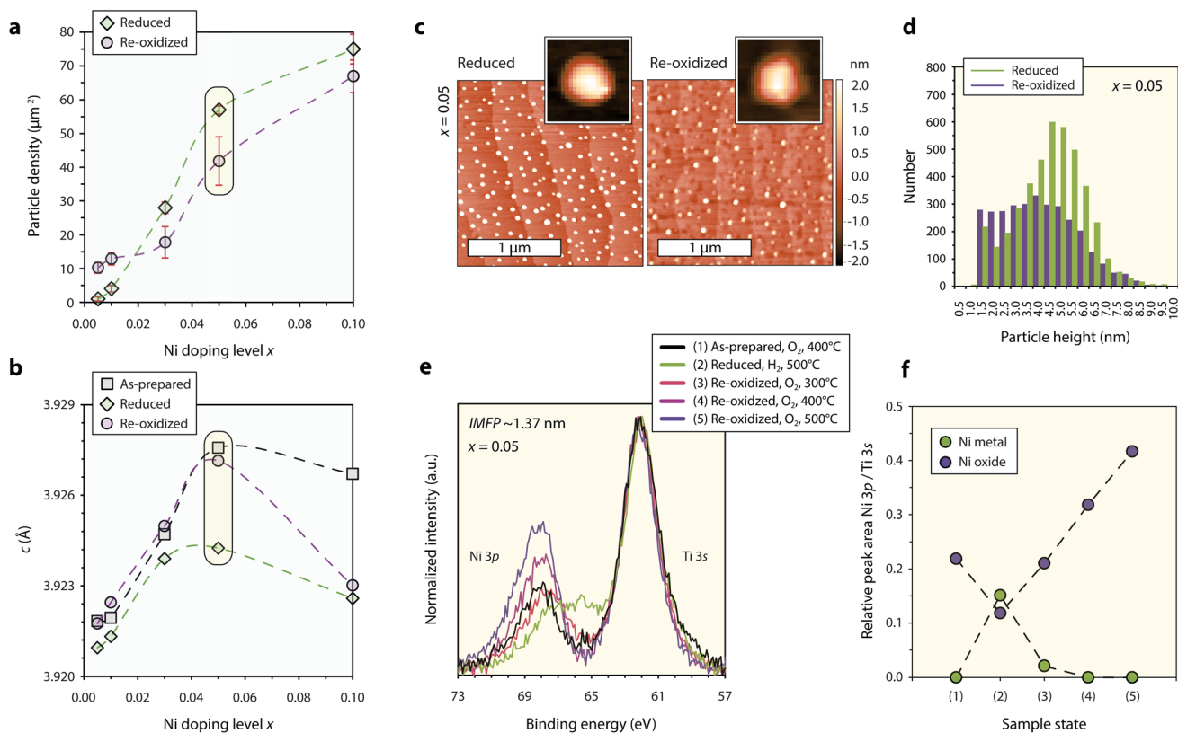
Fig. 3 Characterization of the redox response of epitaxial STNNix thin films. (a) Nanoparticle density detected for STNNix ( x = 0.005\text{--}0.05 ) by atomic force microscopy using a lower threshold of 1 nm. The error bars denote the standard deviation of average values obtained by the measurement of three different 5 \times 5 \mu\text{m}^2 scans. (b) Out-of-plane c -lattice parameter of the as-prepared, reduced and reoxidized thin films determined from the position of the (004) diffraction peak obtained from STNNix thin films ( x = 0.005\text{--}0.05 ). (c) Atomic force microscopy images of STNNix ( x = 0.05 ) in the reduced and in the reoxidized states. A single particle image cut from the larger scans is shown as the inset image, respectively. (d) Frequency distribution of the maximum height of exsolved nanoparticles after reduction and reoxidation determined on the basis of three 5 \times 5 \mu\text{m}^2 scans. For (a–d) the reduction step was performed ex situ in continuous flow of a 4% \text{H}_2/\text{Ar} gas mixture at T = 800^\circ\text{C} while the reoxidation step was performed in air at T = 800^\circ\text{C} . (e) Ambient-pressure X-ray photoelectron spectroscopy of the Ni 3p–Ti 3s core-level region obtained from STNNix ( x = 0.05 ). The core-level signature is compared in situ after consecutive oxidation, reduction and reoxidation steps at different temperatures. The hydrogen and oxygen partial pressures were p(\text{H}_2) = 0.5 mbar and p(\text{O}_2) = 0.5 mbar. The binding energies of all spectra were aligned to Ti 2p = 458.4 eV and a Shirley-type background was subtracted. (f) Relative Ni 3p/Ti 3s peak area ratio derived from (e) based on deconvolution of the spectra by peak fitting as specified in the ESI.† Yellow boxes in (a and b) highlight data points obtained from STNNix ( x = 0.05 ). Dashed lines serve as a guide for the eye.
