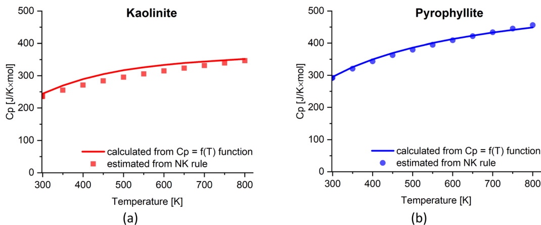
Fig. 5 The estimated C_p value of (a) kaolinite and (b) pyrophyllite based on NK rule compared with the C_p = f(T) function. 41
