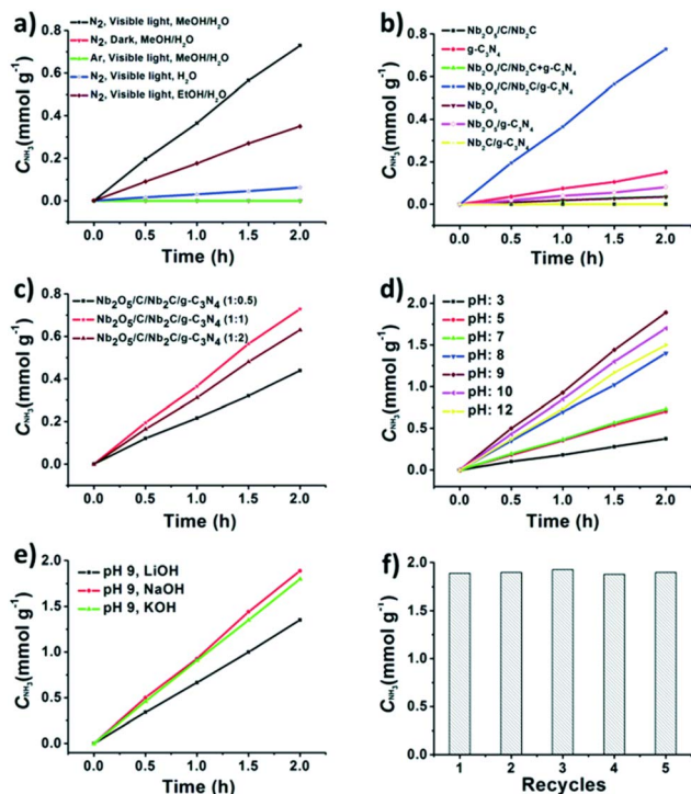
Fig. 13 (a) Control experiments on photocatalytic \text{NH}_3 production with the MXene-derived \text{Nb}_2\text{O}_5/\text{C}/\text{Nb}_2\text{C}/\text{g-C}_3\text{N}_4 heterojunction under different conditions. (b) Photocatalytic activity of the \text{Nb}_2\text{O}_5/\text{C}/\text{Nb}_2\text{C} , \text{g-C}_3\text{N}_4 , \text{Nb}_2\text{O}_5/\text{C}/\text{Nb}_2\text{C} + \text{g-C}_3\text{N}_4 , \text{Nb}_2\text{O}_5/\text{C}/\text{Nb}_2\text{C}/\text{g-C}_3\text{N}_4 , \text{Nb}_2\text{O}_5 , \text{Nb}_2\text{O}_5/\text{g-C}_3\text{N}_4 and \text{Nb}_2\text{C}/\text{g-C}_3\text{N}_4 for \text{NH}_3 production under visible light irradiation ( \lambda > 420 nm). (c) Photocatalytic \text{NH}_3 production activity of \text{Nb}_2\text{O}_5/\text{C}/\text{Nb}_2\text{C}/\text{g-C}_3\text{N}_4 with the ratio variation of \text{Nb}_2\text{O}_5/\text{C}/\text{Nb}_2\text{C} : melamine from 0.5 to 1 and 2 during catalyst preparation; (d) photocatalytic \text{NH}_3 production activity of \text{Nb}_2\text{O}_5/\text{C}/\text{Nb}_2\text{C}/\text{g-C}_3\text{N}_4 with different pH values adjusted by using HCl or NaOH solution. Reproduced with permission from ref. 157, Copyright 2020 The Royal Society of Chemistry.
