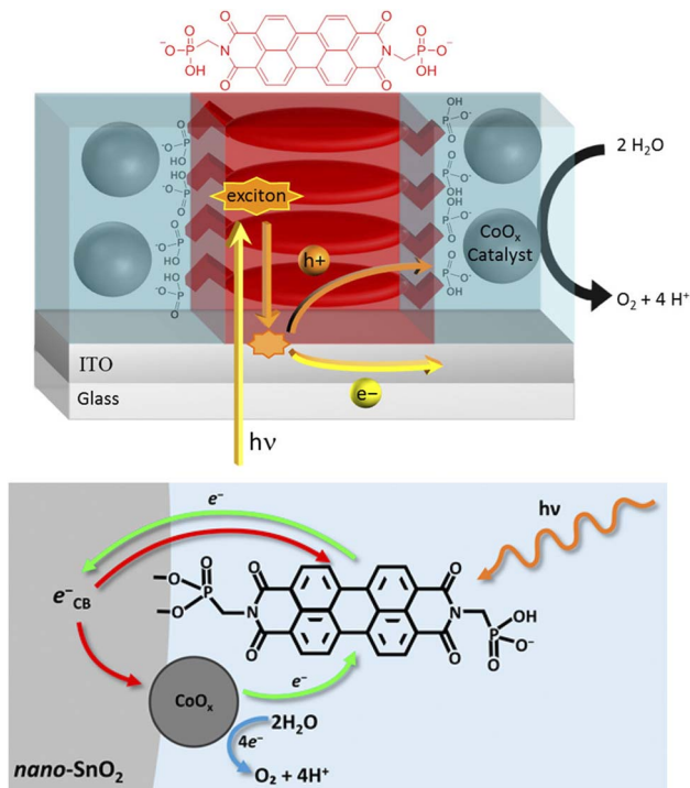
Fig. 15 Perylene bisimide (PBI) photosensitizers combined with a cobalt oxide WOC onto ITO or mesoporous SnO 2 , developed by Finke and co-workers. Reprinted from ref. 111 and 112 with permission from the American Chemical Society, copyright 2017 and 2022.
