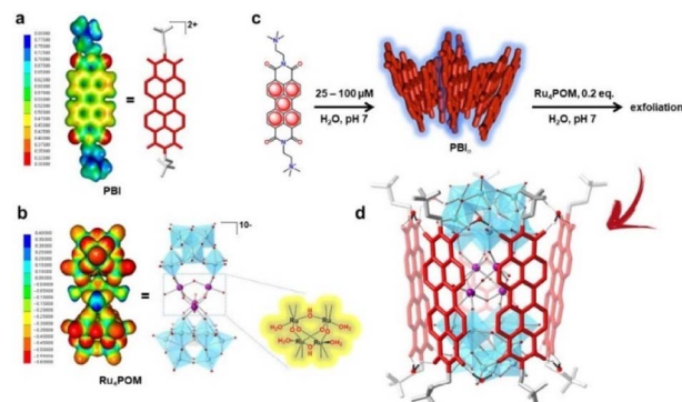
Fig. 17 Self-assembly in water of artificial quasomes (QS) from a dicationic perylene bisimide \text{PBI}^{2+} and a decaanionic \text{Ru}_4\text{POM} WOC. Reprinted from ref. 117 with permission from the Nature Publishing Group, copyright 2019.
