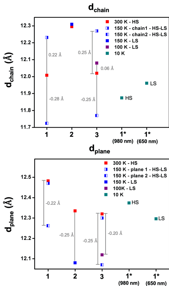
Fig. 4 Plots of the variation of the d_{\text{chain}} (top) and d_{\text{plane}} (bottom) for 1 , 2 , and 3 at different temperatures. The changes in these values are indicated by the grey bars. * indicates irradiated samples.
