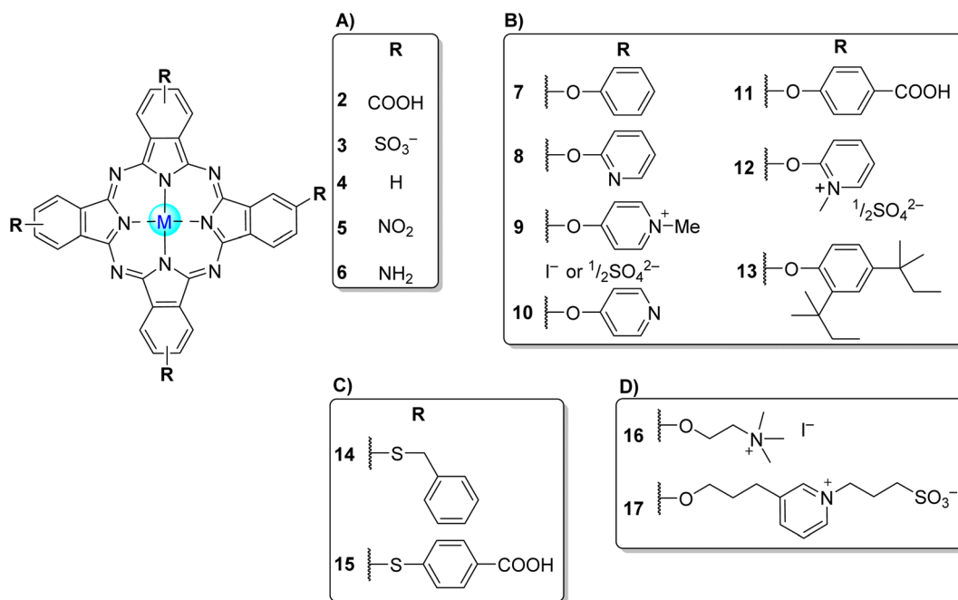
Fig. 4 Symmetrical tetra-β-substituted phthalocyanines (A) 2–6, 34,45–96 (B) 7–13, 84,85,97–100 (C) 14, 50,101 15 35,101 and (D) 16, 56,85 17. 102
