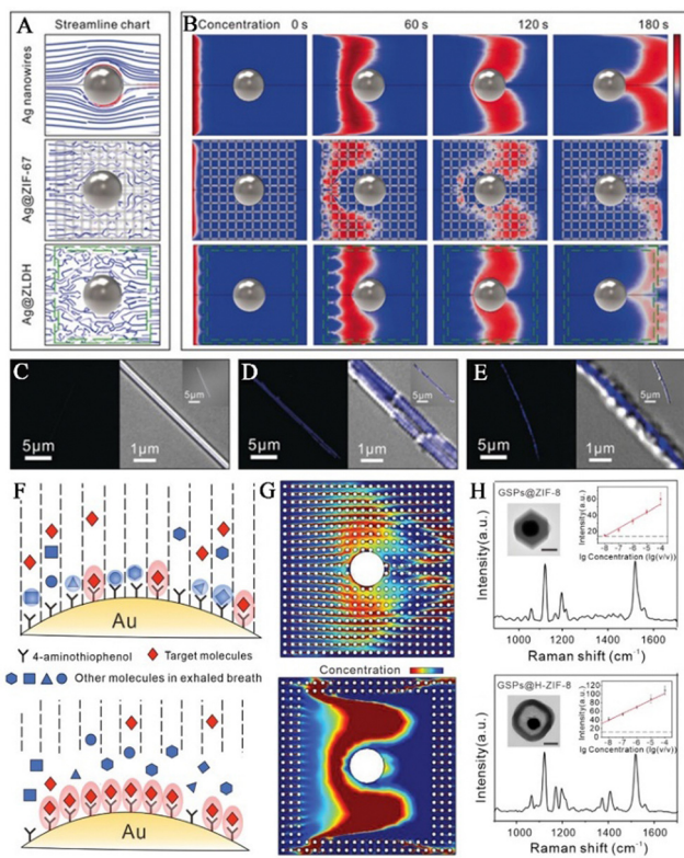
Fig. 8 MOFs for preconcentration of analytes. (A) Simulation streamline graphs of Ag nanowires, Ag@ZIF-67, and Ag@LDH. (B) Modeling fluctuations in the concentrations of Ag nanowires, Ag@ZIF-67, and Ag@LDH through simulations. (C–E) The confocal microscopy images of surface adsorption of fluorescent gaseous molecules experiment: (C) Ag wires, (D) Ag@ZIF-67, and (E) Ag@LDH. Inset: the fluorescence image and overlays of fluorescence and transmission images. 41 Reproduced with permission from John Wiley and Sons, copyright 2019. (F) Illustration showing the adsorption process between molecules in exhaled gas and various substrates. (G) Modeling the variation in concentrations of GSPs@ZIF-8 and GSPs@H-ZIF-8 through simulations. (H) Simulations of alterations in the concentrations of GSPs@ZIF-8 and GSPs@H-ZIF-8. Inset: TEM images of GSPs@ZIF-8 and GSPs@H-ZIF-8. 40 Reproduced with permission from John Wiley and Sons, copyright 2022.
