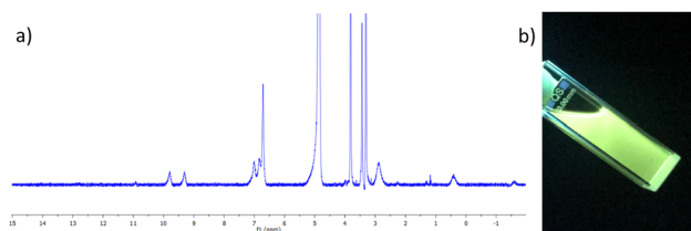
Fig. 2 (a) The 1 H NMR spectrum (400 MHz, CD 3 CN- d 3 ) of [Tb( 3 ) 3 ](CF 3 SO 3 ) 3 showing significant shift and broadening of the signals relative to the free ligand 3 (see ESI† for NMR). (b) The bright green Tb(III) emission arising from the 3.Tb complex in CH 3 CN under UV-light (λ ex = 254 nm).
