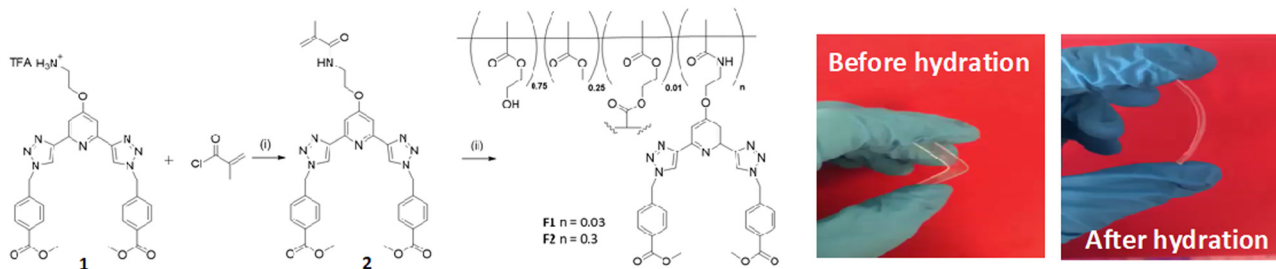
Scheme 1 Synthesis and structure of monomer 2 , formed from ligand 1 , and the two polymeric films F1 and F2 . Reagents and conditions: (i) NEt 3 , CH 2 Cl 2 (ii) 80 °C 6 hours. F1 (0.03 wt%) and F2 (0.3 wt%), respectively. Pictures show the films formed before and after being hydrated.
