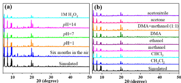
Fig. 3 PXRD pattern of \text{Cu}_{12} showing the stability under different conditions: (a) in air and water solution; (b) in common organic solvents.
