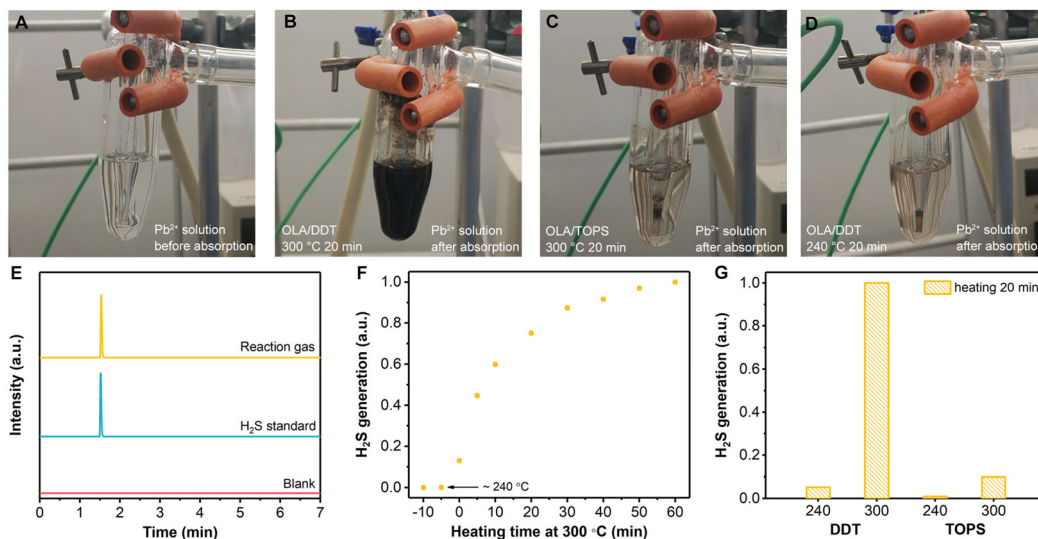
Fig. 3 (A–D) Detection of H_2S gas generation by Pb^{2+} aqueous solution. (A) Pb^{2+} solution before reaction. (B–D) Pb^{2+} solution after absorption under different reaction conditions: (B) OLA/DDT at 300 °C, (C) OLA/TOPS at 300 °C, and (D) OLA/DDT at 240 °C. (E–G) Detection of H_2S gas generation by GC-FPD. (E) Comparison between the gas extracted from the flask, H_2S standard gas ( H_2S in Ar) and blank (Ar). (F) Time monitoring of H_2S gas generation from DDT and OLA during heating at 300 °C. The time before 0 min represents the heating-up period. (G) Comparison of H_2S generation under different reaction conditions.
