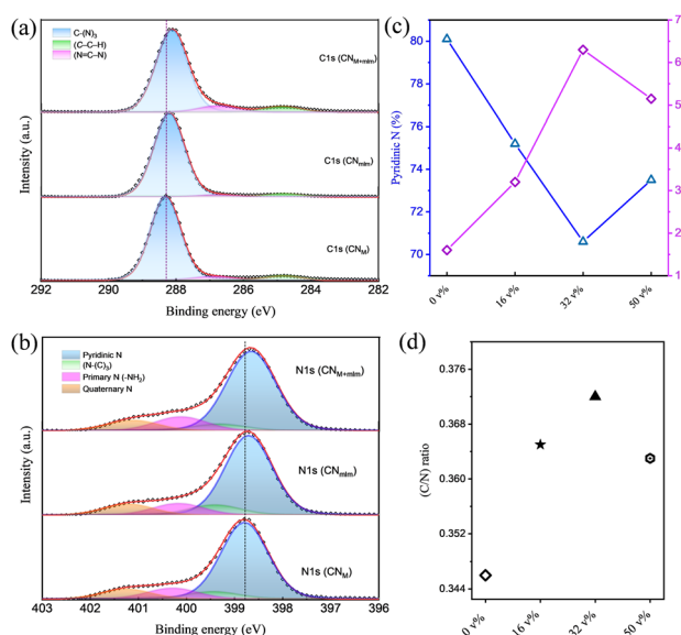
Fig. 4 XPS CN analysis. High-resolution (a) C 1s and (b) N 1s XPS spectra of \text{CN}_M , \text{CN}_{M+mlm} , and \text{CN}_{M+mlm} . (c) Calculated percentage of pyridinic N and free \text{NH}_2 species for various amounts of EG (v%) used in the hydrothermal treatment during \text{CN}_{M+mlm} syntheses, calculated from N 1s spectra. (d) Atomic C/N ratio obtained from survey scans of \text{CN}_{M+mlm} prepared with varying EG content. The experimental points in (a) and (b) are fitted with a red line, which is deconvoluted into peaks corresponding to the indicated chemical species. The lines connecting the diamonds and triangles in (c) serve as a guide to the eye.
