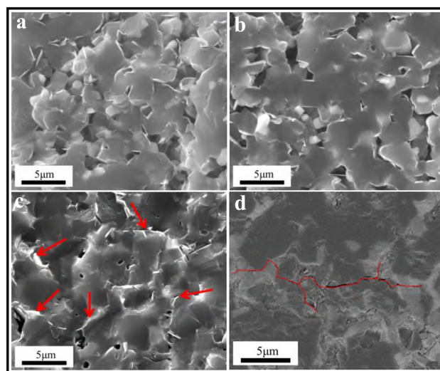
Fig. 15 Fracture surfaces of hot-press sintered B_4C -20 wt% SiC ceramics produced at different sintering pressures: (a) 30 MPa, (b) 35 MPa, and (c) 40 MPa. 122 (d) Indentation crack deflection in hot-press sintered B_4C -20 wt% SiC ceramics produced at a sintering pressure of 40 MPa. 122
