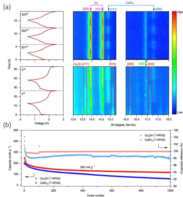
Fig. 8 (a) Isoplots of in situ XRD scans the anode Ca x Sn||14PAQ cells during the first, second and from 201st to 203rd discharge/charge cycles at specific current of 26 mA g -1 at 25 °C. The peak is observed along the top and the cell voltage profiles on the left had side. ICSD-ID: Ca 2 Sn 659 611, β-Sn 106 072, CaSn 3 58 934, Ca 36 Sn 23 54 619 and CaO 26 959. (b) Cycling performance of CaSn 3 ||14PAQ compared with Ca x Sn||14PAQ. Reproduced with permission from ref. 94, copyright 2022 Springer Nature.
