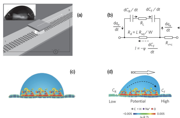
Fig. 2 Mechanism of charge separation on graphene. (a) Illustration of the experimental set-up. A liquid droplet is sandwiched between graphene and a \text{SiO}_2/\text{Si} wafer, and drawn by the wafer at specific velocities. Inset: A droplet of 0.6 M NaCl solution on a graphene surface with advancing and receding contact angles of 91.98^\circ and 60.28^\circ , respectively. (b) Equivalent circuit for (d). (c) Schematic illustration of the pseudo-capacitance formed by a static droplet on graphene. (d) Schematic illustration of the potential difference induced by a moving droplet (figures and captions reproduced from ref. 19 with permission from Springer Nature, copyright 2014).
