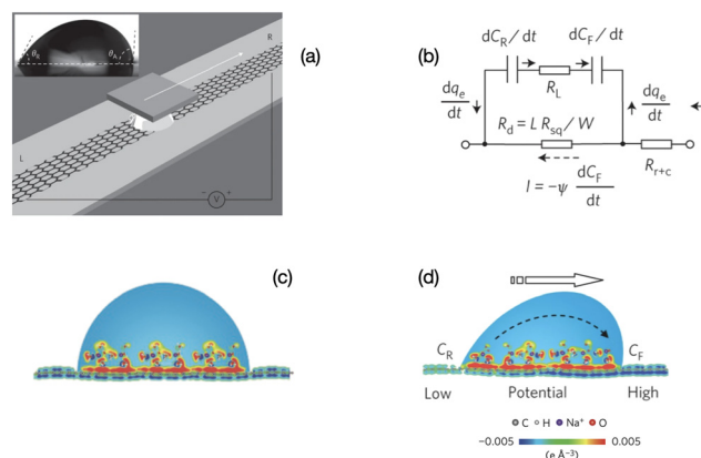
Fig. 2 Mechanism of charge separation on graphene. (a) Illustration of the experimental set-up. A liquid droplet is sandwiched between graphene and a SiO 2 /Si wafer, and drawn by the wafer at specific velocities. Inset: A droplet of 0.6 M NaCl solution on a graphene surface with advancing and receding contact angles of 91.98° and 60.28°, respectively. (b) Equivalent circuit for (d). (c) Schematic illustration of the pseudo-capacitance formed by a static droplet on graphene. (d) Schematic illustration of the potential difference induced by a moving droplet (figures and captions reproduced from ref. 19 with permission from Springer Nature, copyright 2014).
