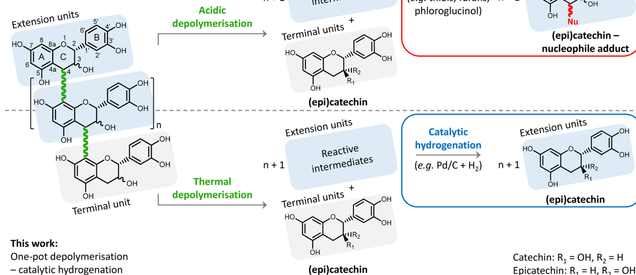
Fig. 1 Comparison of the proposed one-pot depolymerisation–hydrogenation of condensed tannins, with the state-of-the-art one-pot depolymerisation – nucleophilic trapping. Above: common acidic depolymerisation combined with nucleophilic trapping forming adducts from ( epi )catechin rather than ( epi )catechin itself. Below: thermal depolymerisation combined with catalytic hydrogenation, leading to ( epi )catechin. A general procyanidin structure is shown on the left, with the numbering indicated on one of its monomers.
