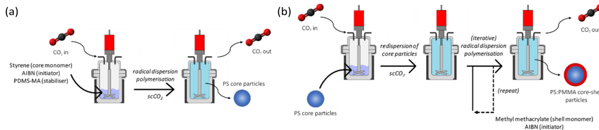
Fig. 1 Reaction schematic of (a) PS core and (b) PMMA shell syntheses in supercritical \text{CO}_2 in a high-pressure autoclave.
