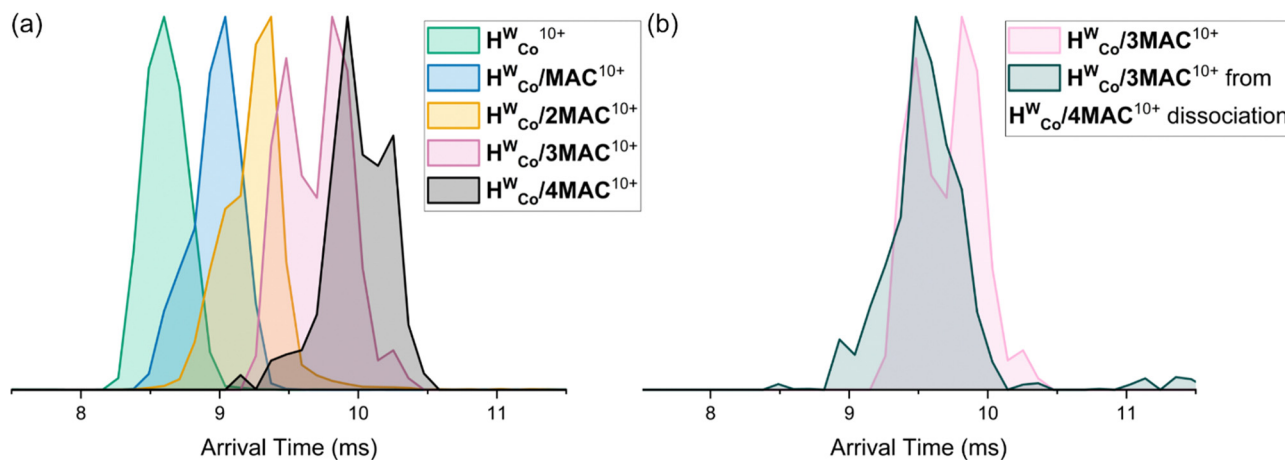
Fig. 5 (a) ATDs of H_{Co}^W/nMAC^{10+} with n = 1-4 . (b) ATDs of 'free' H_{Co}^W/3MAC^{10+} and H_{Co}^W/3MAC^{10+} formed purely from dissociation of H_{Co}^W/4MAC^{10+} .
