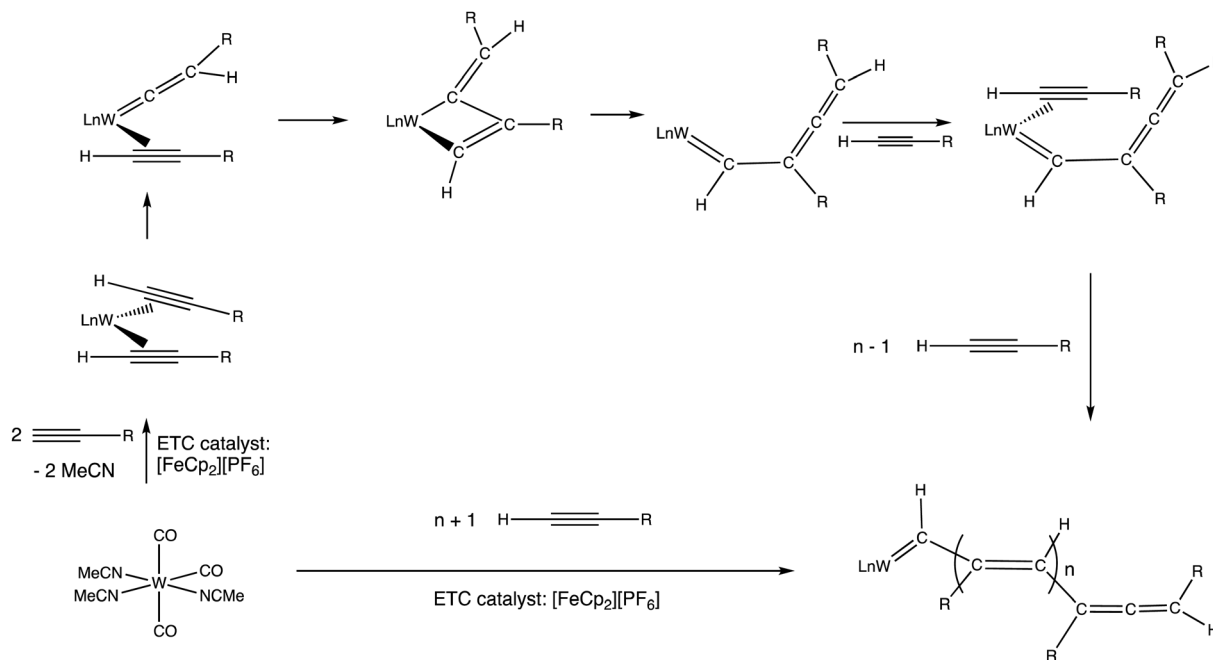
Scheme 4 Polymerization of terminal alkyne catalyzed by a \text{W}(0) pre-catalyst according to the Chauvin–Katz metathesis mechanism. Addition of a catalytic amount of [\text{FeCp}_2][\text{PF}_6] vs. the \text{W}(0) catalyst considerably accelerates the reaction (from 100 °C, hours, in the absence of [\text{FeCp}_2][\text{PF}_6] to r.t. within a few minutes. Exchange of MeCN by the alkyne in the 18-electron \text{W}(0) complex is slow, but it becomes very fast at the 17-electron level. Following this exchange, the ETC cross redox step with the starting pre-catalyst is also fast due to its exergonicity, because the alkyne is a \pi -acceptor, contrary to MeCN. 36
