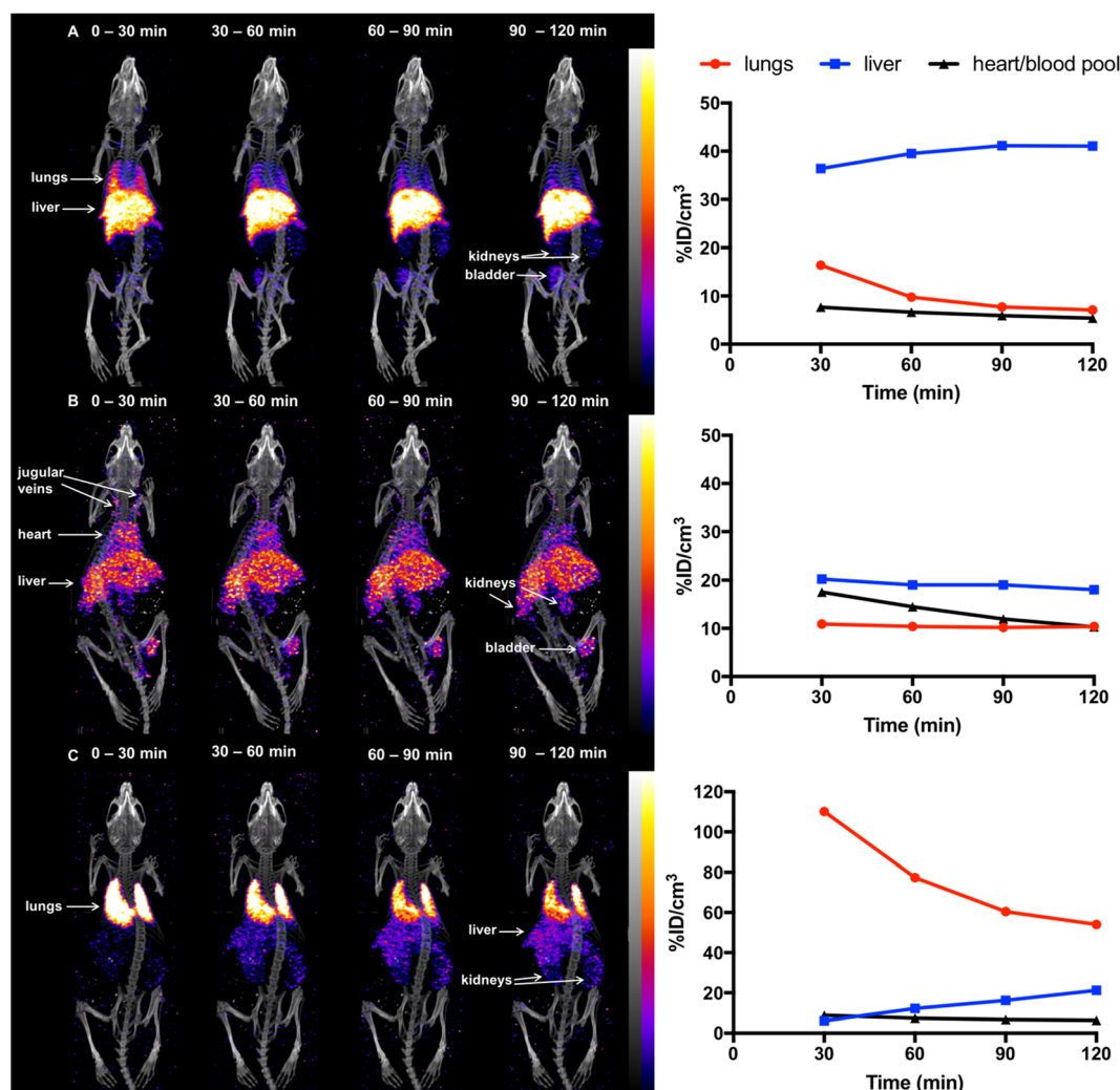
Fig. 3 SPECT/CT maximum intensity projections and ^{111}\text{In} concentrations in specific organs for mice administered (a) [ ^{111}\text{In} ]In-DTPA-CTP-labelled 5T33 cells (SPECT scale of 0.8–8 \% \text{ID g}^{-1} ), (b) [ ^{111}\text{In} ]In-DTPA-CTP (cell-free) (SPECT scale of 1.6–8 \% \text{ID g}^{-1} ) and (c) [ ^{111}\text{In} ]In-(oxine) 3 -labelled 5T33 cells (SPECT scale of 1.6–16 \% \text{ID g}^{-1} ), acquired 0–30 min, 30–60 min, 60–90 min and 90–120 min post-injection.
