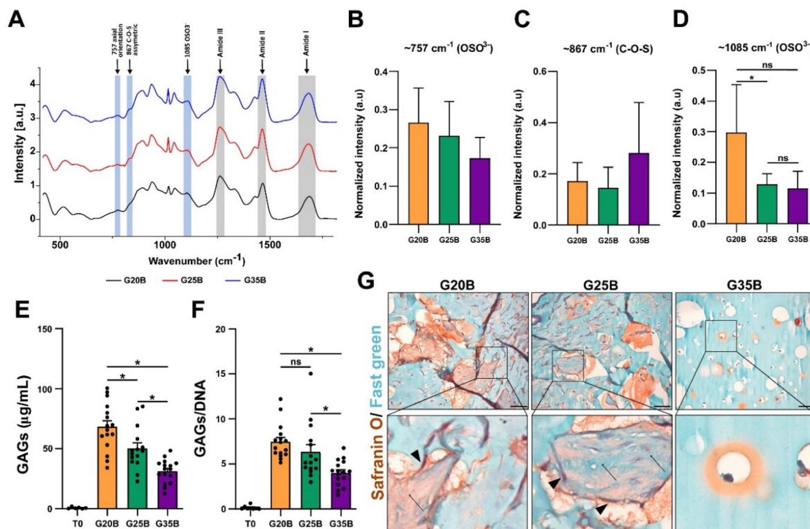
Fig. 6 Encapsulated OACs synthesize GAGs in a stiffness-dependent way. (A) The spectra of samples were analyzed in the 350–1800 cm -1 range to detect molecular vibrations of the C4S sulfated groups present in GAGs. Bands from amide groups are depicted in gray bars and the vibration from C4S bonds is in light blue. These data are shown comparing the spectra from day 35 to day 0 and then were normalized internally to compare different formulations and plotted as arbitrary units (a.u.). Quantification of main bands for GAGs in G20B, G25B, and G35B at (B) 757, (C) 867, and (D) 1085 cm -1 , n = 3 hydrogels per formulation and 3 OACs donors, (Stratigraphic software was used for statistical analyses, * p < 0.05 ). (E) Biochemical detection of GAGs in hydrogels from day 0 and day 35. (F) GAG data normalized by DNA content. n = 4 hydrogels per formulation and 4 OACs donors, ANOVA test and Dunn's post-test, * p < 0.05 . (G) Safranin O/Fast green staining in hydrogels of G20B, G25B, and G35B after 35 days of differentiation. Scale bar = 50 \mu\text{m} . Arrows indicate protein fibers inside pores and arrow-heads cells in the surrounding.
