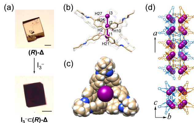
Fig. 5 Anion recognition in (R)- \Delta . (a) Photographs of single crystals of (R)- \Delta and [I 3 - ](R)- \Delta . (b) and (c) Superstructure of [I 3 - ](R)- \Delta in tubular and (c) space-filling representations exhibiting the encapsulation of I 3 - inside the cavity of (R)- \Delta by 18 [C-H...I] interactions. C, tan; N, blue; H, white; I, purple. (d) Side-on (top) and top (down) views of the double helical superstructure of [I 3 - ](R)- \Delta . Hydrogen atoms are omitted for clarity. One strand in the double helix is depicted in orange tubular representation and the other in blue, while I 3 - is represented in a space-filling form.
