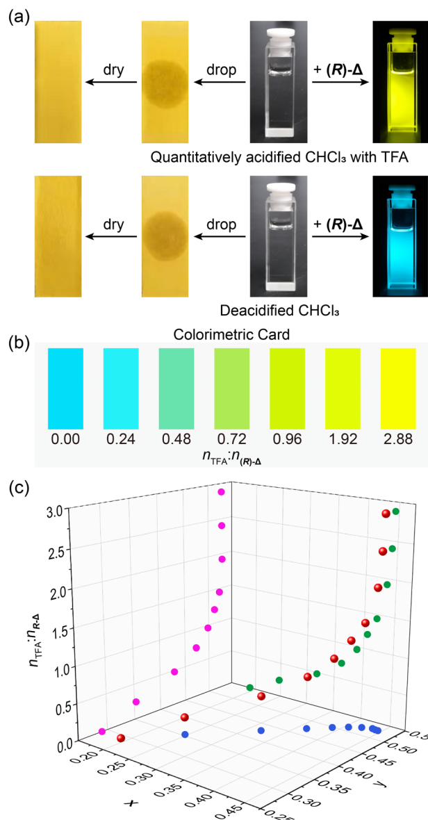
Fig. 4 Detecting traces of acids employing (R)- \Delta . (a) Fluorescence changes of solutions (right) of (R)- \Delta in \text{CHCl}_3 with and without TFA upon shining 365 nm-UV light in comparison with detecting trace acid in the same solvents using pH papers (left). (b) A colorimetric card showing the ability of (R)- \Delta to detect visually amounts of acid in solutions with different n_{\text{TFA}}:n_{(\text{R})-\Delta} ratios. (c) The fitting function based on the PL emission of (R)- \Delta upon changing the n_{\text{TFA}}:n_{(\text{R})-\Delta} ratio from 0.00 to 2.88. The concentration of (R)- \Delta is 1 \times 10^{-5} M.
