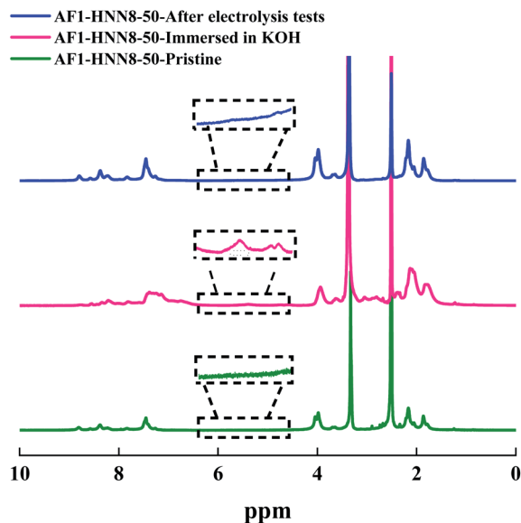
Fig. 6 ^1\text{H} NMR spectra of AEM HNN8-50, in the pristine form (lower), after storage in 2 M KOH at 90 °C for one month (mid), and after the electrolysis test (upper). The data were recorded in DMSO- d_6 .
