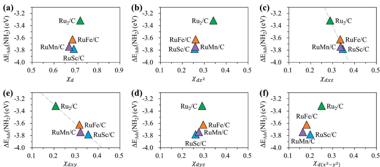
Fig. 11 Relationship between \text{NH}_2 adsorption energy [ \Delta E_{\text{ads}}(\text{NH}_2) ] and orbital overlap [ \chi_d ] for the \text{RuM} (M = Sc, Mn, Fe) DACs (a) \chi_d , (b) \chi_{d_{z^2}} , (c) \chi_{d_{xz}} , (d) \chi_{d_{yz}} , (e) \chi_{d_{xy}} and (f) \chi_{d_{x^2-y^2}} .
