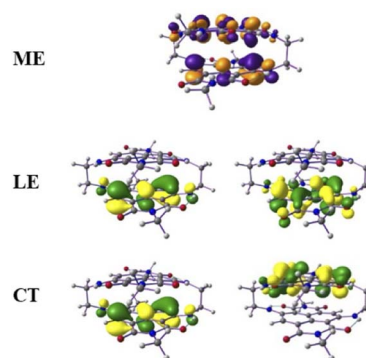
Fig. 4 The molecular orbital (isovalues of \pm 0.04 au) corresponding to the ME configuration in the S_{1a} (dark) state and LE and CT configurations in the S_{2a} (bright) state.
