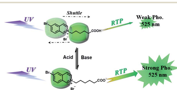
Fig. 5 Schematic illustration of the construction of a pH-controlled molecular shuttle in aqueous solution based on CB[7] and the 6-bromoisoquinoline derivative.
