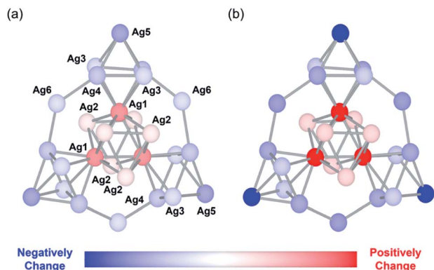
Fig. 4 Schematic of the changes in the natural charge of the \{Ag_{27}\} nanocluster of Ag_{27} upon protonation. Change in the natural charge of each Ag atom after adding (a) three additional protons and (b) six additional protons to the polyoxometalate (POM) frameworks. Silver atoms are colored according to the changes in the natural charges with respect to those of Ag_{27} . The POM frameworks are omitted for clarity (see Fig. S4 in ESI† for the total anion structure of Ag_{27} including POM frameworks).
