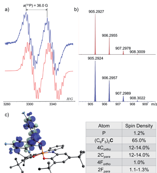
Fig. 7 (a) EPR spectra of [1\text{-OC(C}_6\text{F}_5)_2]^\bullet (blue) and its simulation (red); (b) MS of the reduced [1\text{-OC(C}_6\text{F}_5)_2]^\bullet ( 905.2927 (M) ^\bullet ) (red) and its simulation (blue); (c) DFT calculated Mulliken atomic spin densities in [1\text{-OC(C}_6\text{F}_5)_2]^\bullet .
