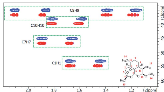
Fig. 2 A portion of the CLIP-HSQC spectrum of artemether 1 in the isotropic \text{CD}_3\text{OD} medium (red) and anisotropic OPA-1 phase (blue).
