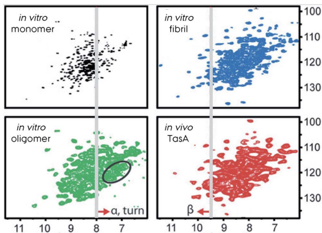
Fig. 3 (A) Representation of bacteria mediated biofilm formation, initiated by the motile species gathering together into the mature solid biofilm matrix. The molecular details of the biofilm composed of bacteria themselves, polysaccharides, extracellular DNA and protein amyloid fibrils are additionally shown. This figure is reproduced with permission. 9 (B) The wild-type (WT) versus the deletion-mutants ( \Delta ) of B. subtilis bacteria and the biofilm formed by them. The WT, \Delta eps, \Delta tasA and \Delta eps-tasA. The deletion mutants form bacterial communities that are healthy but with a weakened/disrupted biofilm. This figure is reproduced with permission. 63 (C) Reconstruction of a native-like B. subtilis biofilm from a \Delta tasA deletion mutant that cannot form biofilm by itself. The supplementation of recombinantly produced TasA protein to the growth medium of the \Delta tasA mutant B. subtilis strain reconstitutes the native-like biofilm. This allows incorporation of isotope-labelled TasA into the biofilm for in vivo NMR spectroscopy without any background signal. (D) 2D ^1\text{H} - ^{15}\text{N} NMR spectra of different TasA samples prepared in vitro , soluble monomer, oligomer and fibril, as well as in vivo TasA in biofilm. Spectral differences indicate structural differences and shed light on the biofilm TasA form. For more details on the figure and explanation of the additional indications, the reader is referred to the original article. This figure is reproduced with permission. 81
