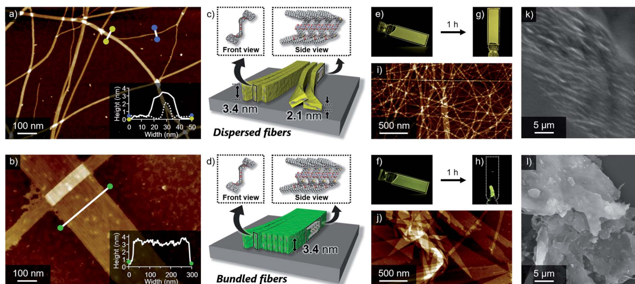
Fig. 3 (a) and (b) AFM images of (a) 1 and (b) 2 aggregates formed in 90 : 10 MCH/CHCl 3 mixture ( c = 100 μM). Insets show cross-section analysis between the yellow dots (solid line), blue dots (dash line) and green dots in the image of (a) and (b), respectively. (c) and (d) Schematic representation of tape-like supramolecular fibers of (c) 1 and (d) 2 with different bundling tendency. (e) and (f) Photographs of as-prepared viscous liquids of (e) 1 and (f) 2 in 90 : 10 MCH/CHCl 3 mixture under 365 nm light illumination ( c = 3 mM). (g) and (h) Photographs of (g) gel of 1 and (h) precipitates of 2 under 365 nm light illumination ( c = 3 mM). (i) and (j) AFM images of (i) dried gel of 1 and (j) precipitates of 2 . (k) and (l) SEM images of (k) dried gel of 1 and (l) precipitates of 2 .
