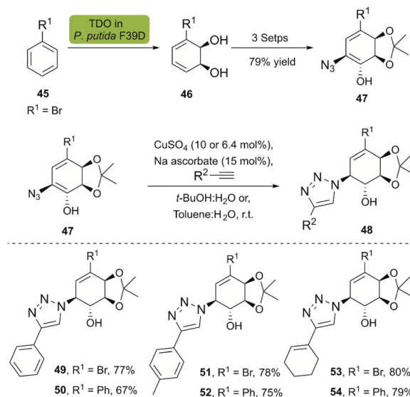
Scheme 5 Chemo-enzymatic synthesis of the bromoazidoconduitrol derivative, and synthesis of triazolyconduitols.
