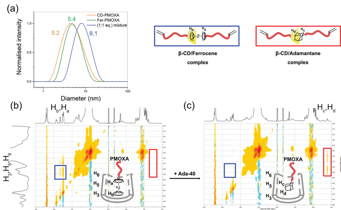
Fig. 3 (a) Size distribution of CD-PMOXA, Fer-PMOXA and their 1:1 molar mixture in at 25 °C ( c = 1 \text{ g mL}^{-1} ). (b) 2D NOESY spectrum of 1:1 molar mixture of CD-PMOXA and Fer-PMOXA ( 5 \text{ mmol L}^{-1} ) in \text{D}_2\text{O} at 30 °C and (c) 2D NOESY spectrum after the addition of Ada-40 (Adamantane-PMOXA).
