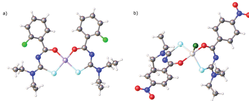
Fig. 4 (a) Molecular structure of [\text{Ni}\{(\text{2-FC}_6\text{H}_4)\text{C}(\text{O})\text{NC}(\text{Se})\text{NEt}_2\}_2] . (b) Molecular structure of [\text{GaCl}\{4\text{-O}_2\text{NC}_6\text{H}_4\text{C}(\text{O})\text{NC}(\text{Se})\text{NEt}_2\}_2] . Atom colours: mint – selenium, blue – nitrogen, red – oxygen, grey – carbon, lilac – nickel, light grey – gallium, light green – fluorine, dark green – chlorine, white – hydrogen.
